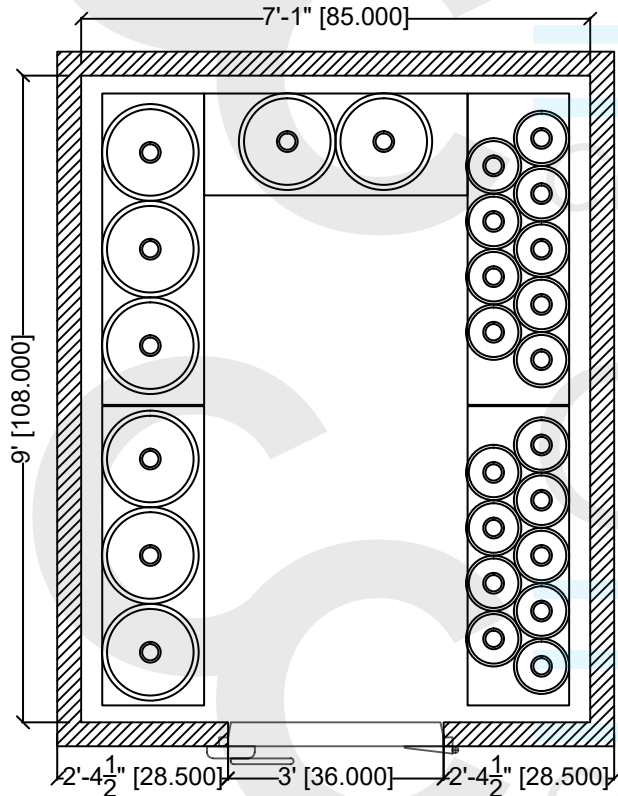
TOP VIEW - MODEL SHOWN: SKS
